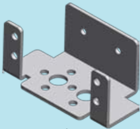
Single Servo Bracket
